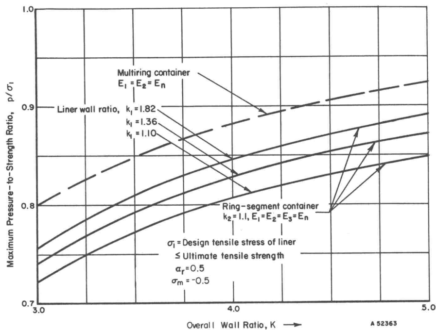
FIGURE 49. COMPARISON OF MULTIRING CONTAINER WITH RING-SEGMENT CONTAINER FOR VARIOUS k_1
